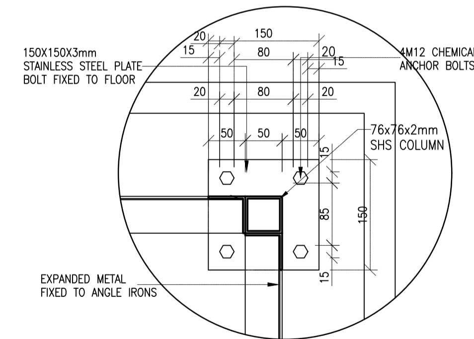
DETAIL B: SECTION OF FIXING PLATE SCALE 1:5
