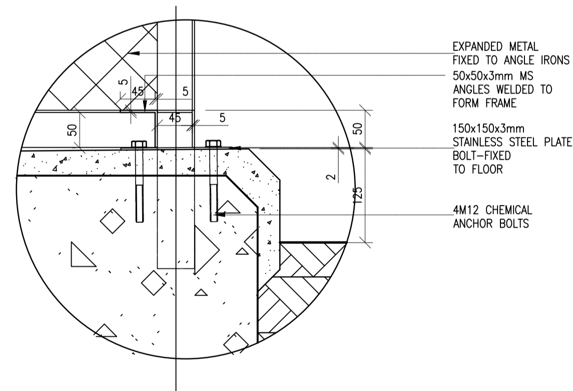
DETAIL A: SECTION OF FIXING PLATE SCALE 1:5
