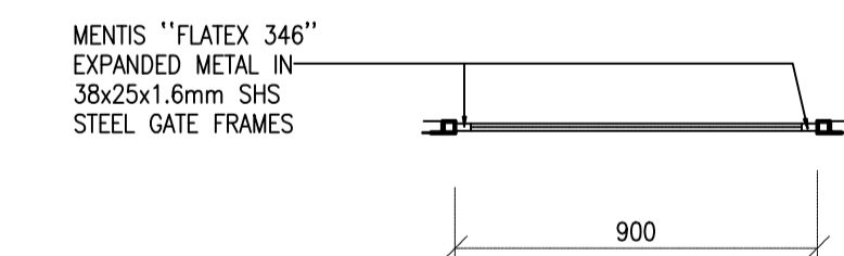
DETAIL C: PLAN OF GATE SCALE 1:20
